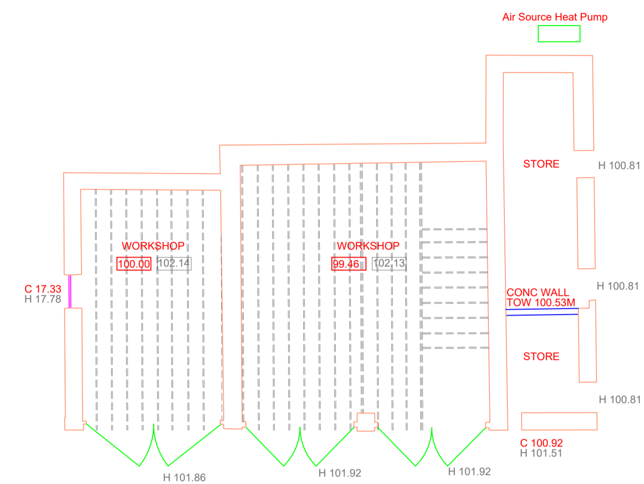
FLOOR PLAN
