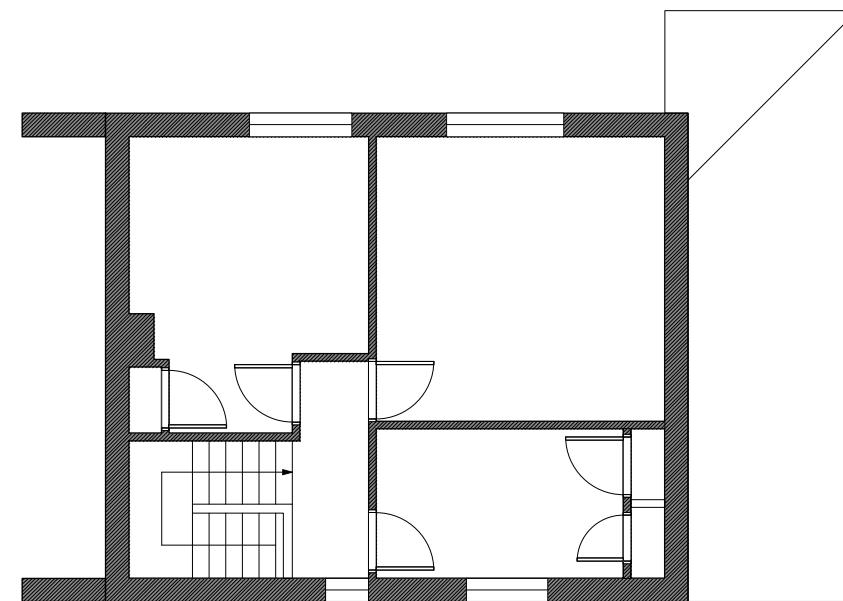
2. First floor plan
