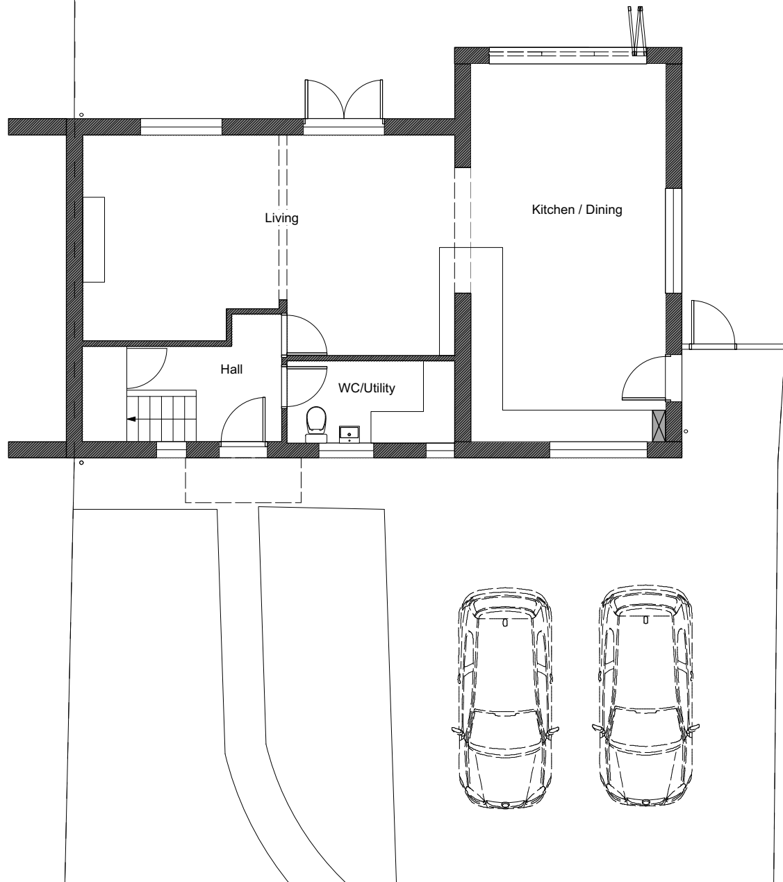
1. Ground floor plan
