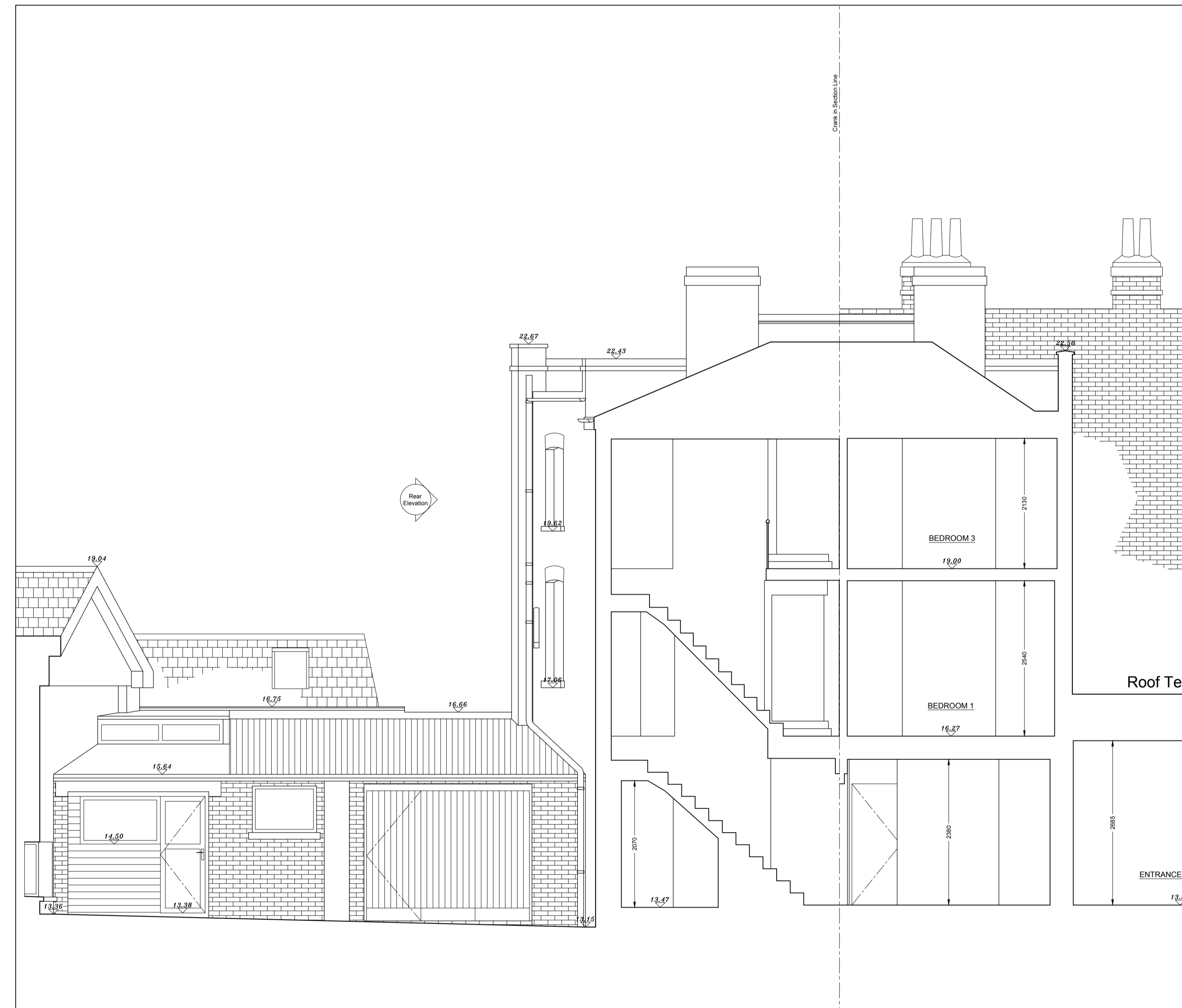
02 Cross Section BB 01-105 SCALE 1:50
