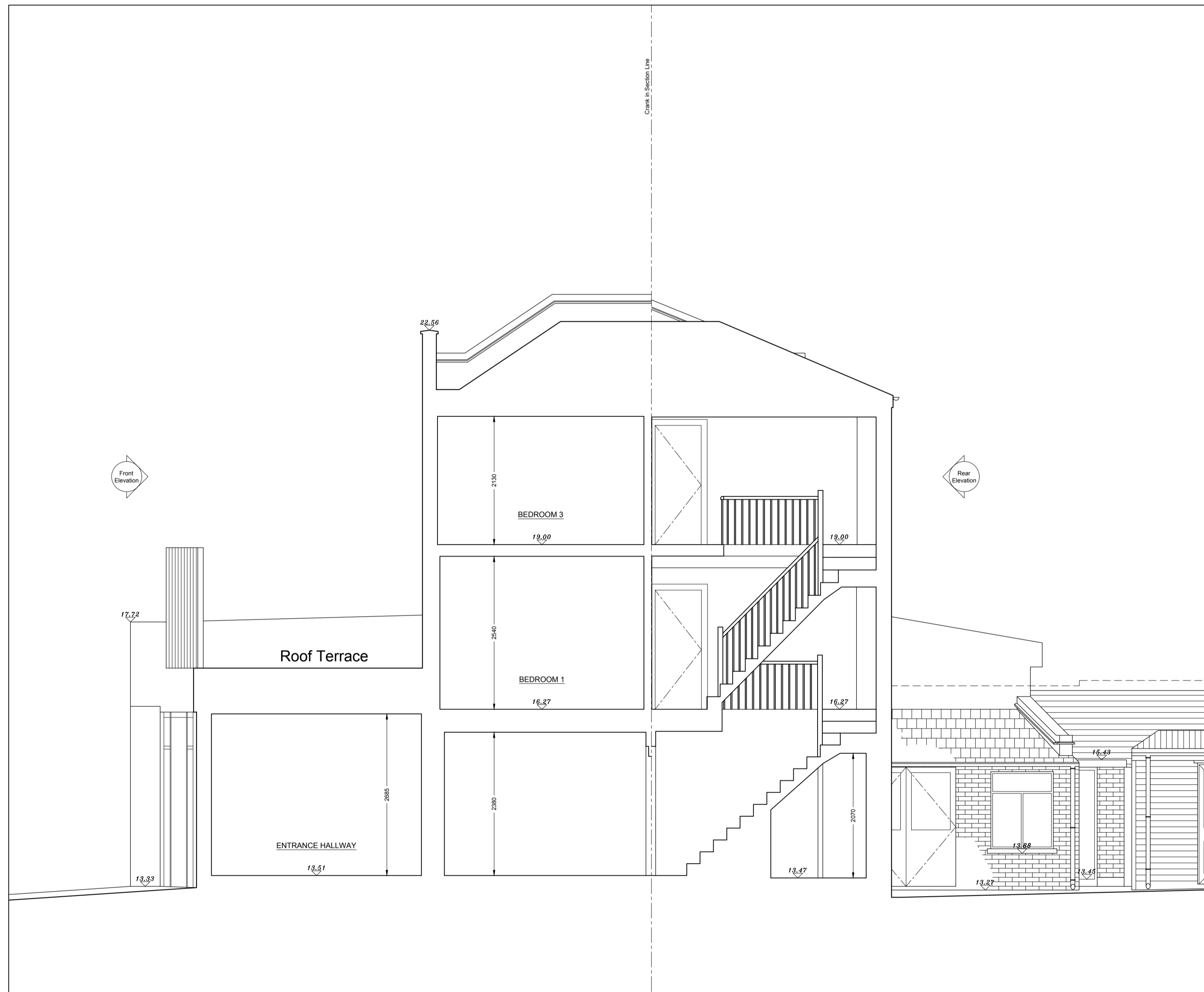
01 Cross Section AA 01-105 SCALE 1:50
