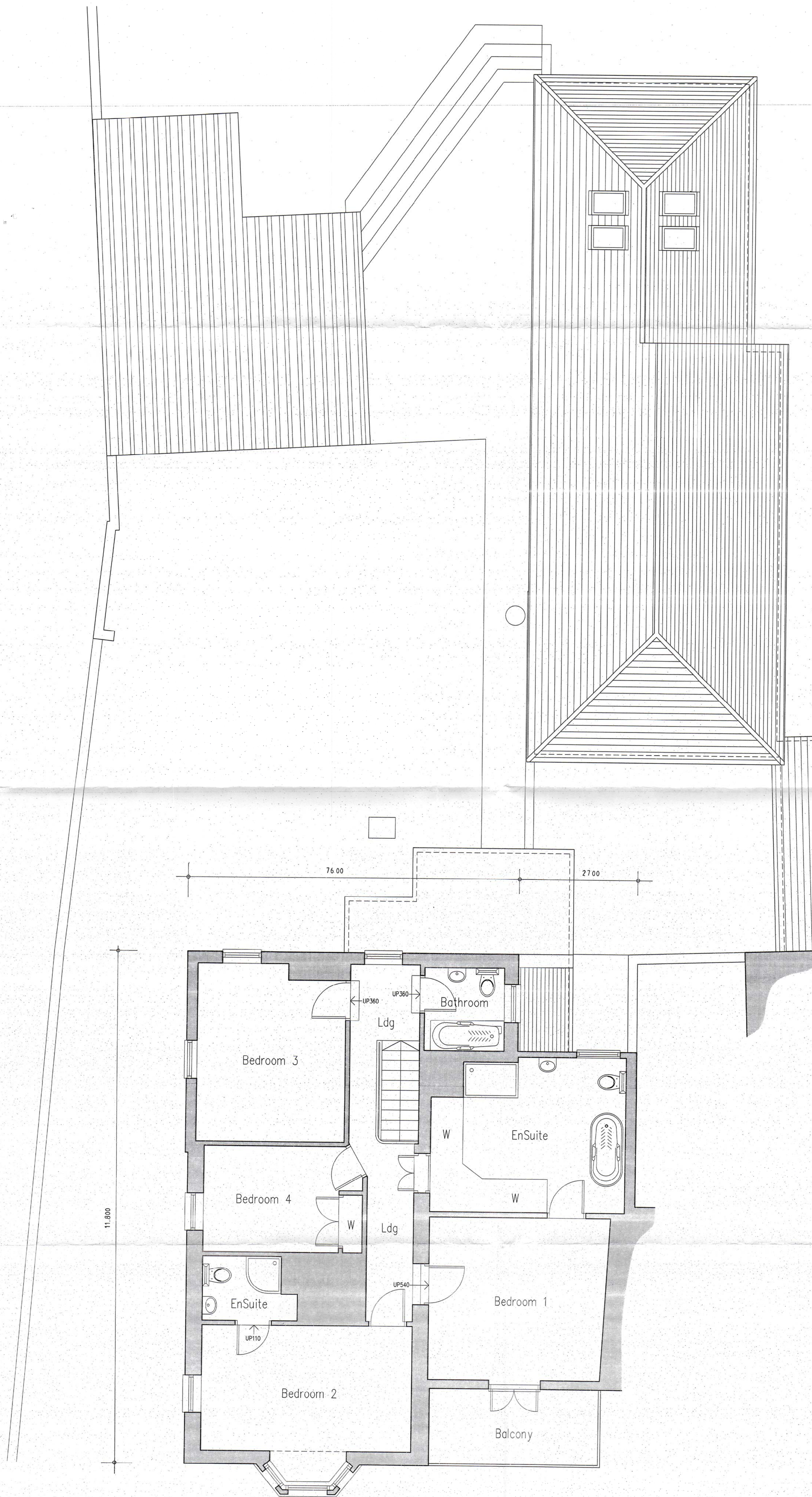
FIRST FLOOR PLAN 1/50 © A1
