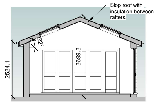
Proposed Family Room Section 1 : 100
