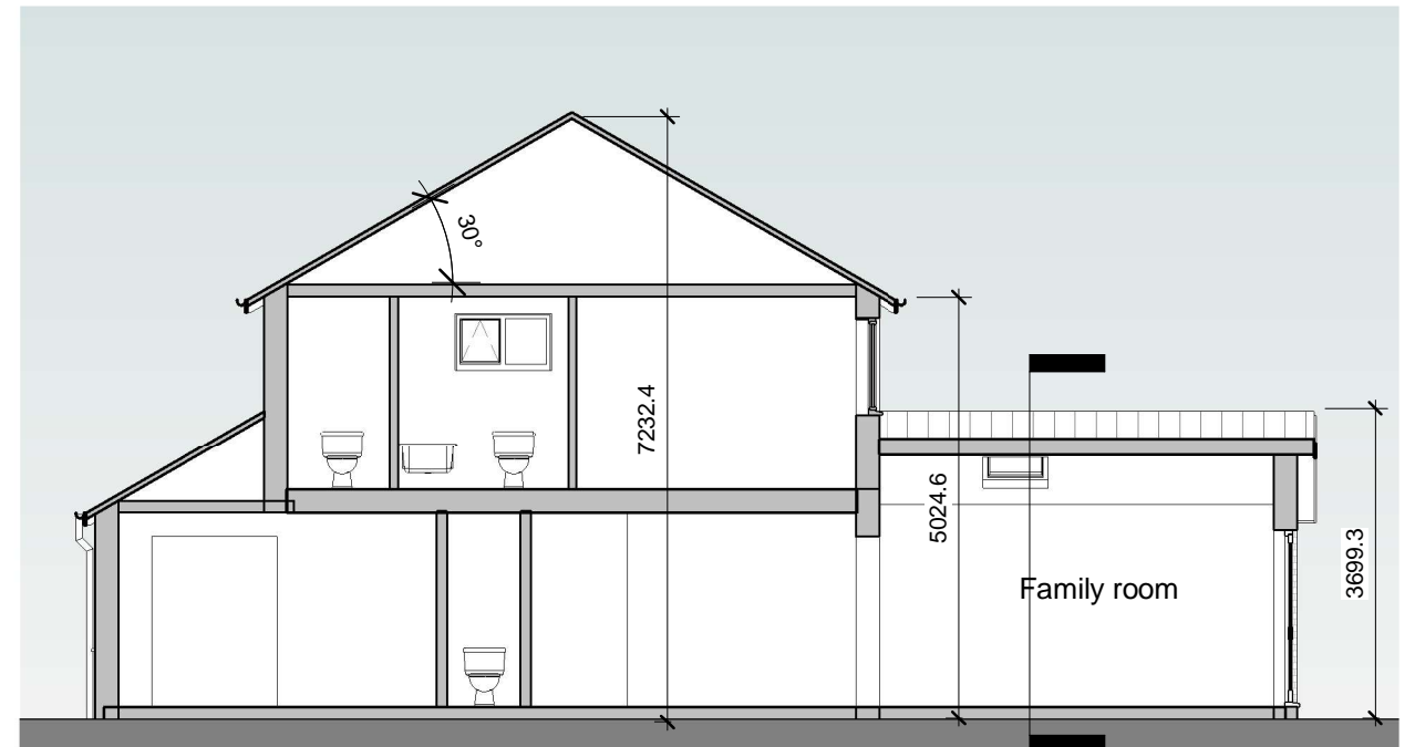
Proposed Section 1 : 100
