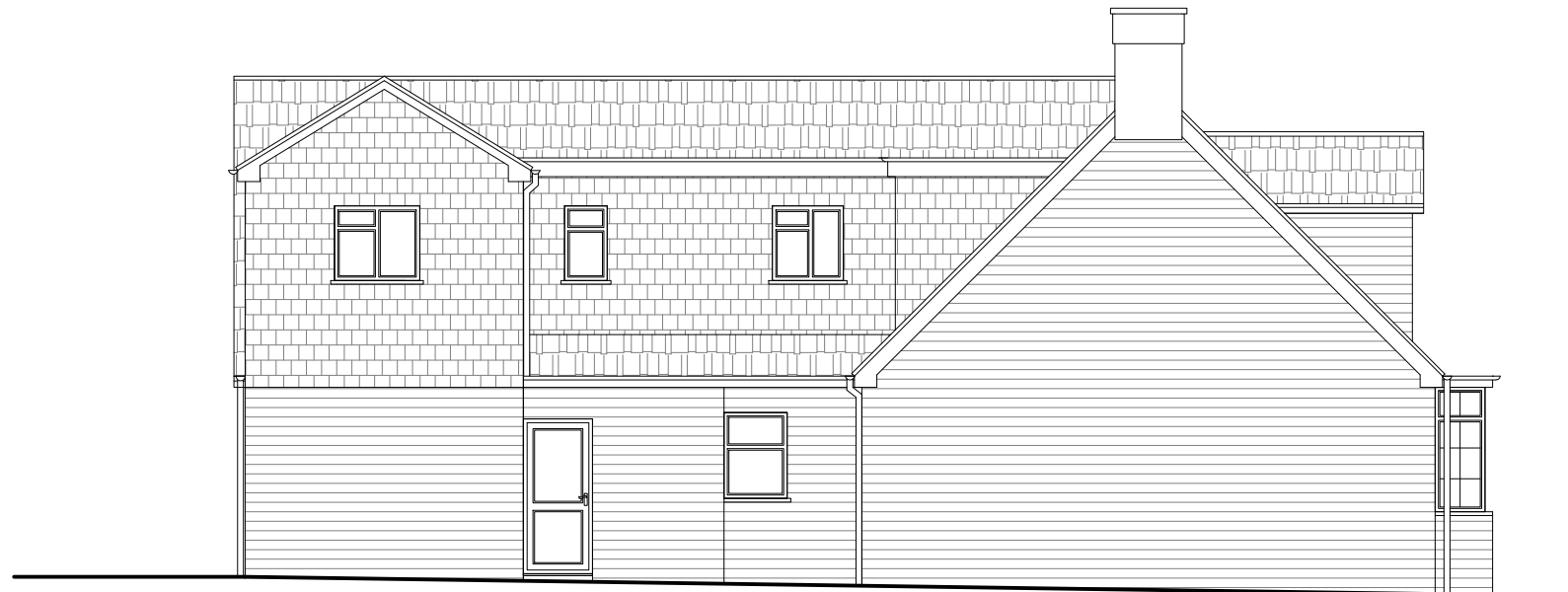
Side Elevation
