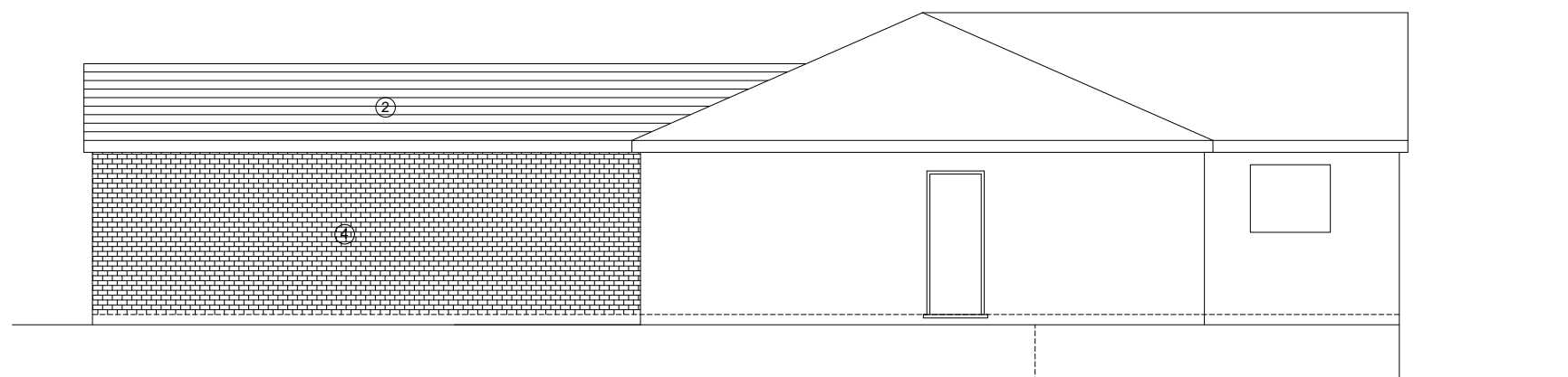
Proposed Side Elevation 4 - 4
