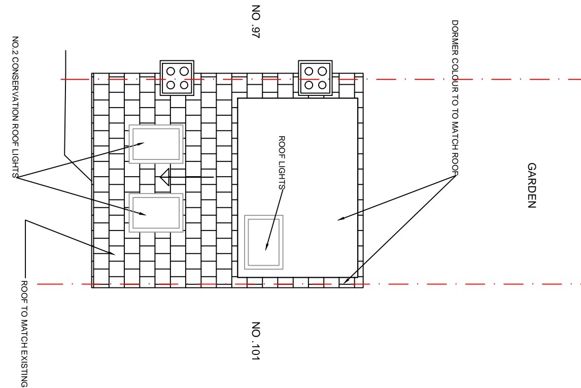
04 Proposed Roof Plan 1:100 (A3)
