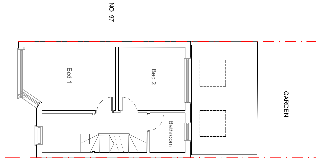
02 Proposed First Floor Plan 1:100 (A3)
