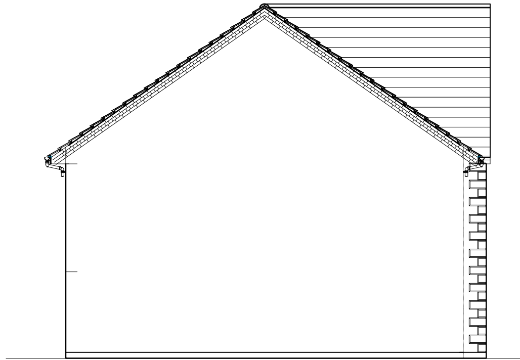
Gable elevation
