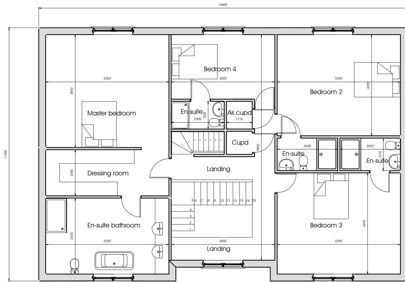
First floor plan Area = 157.37m 2
