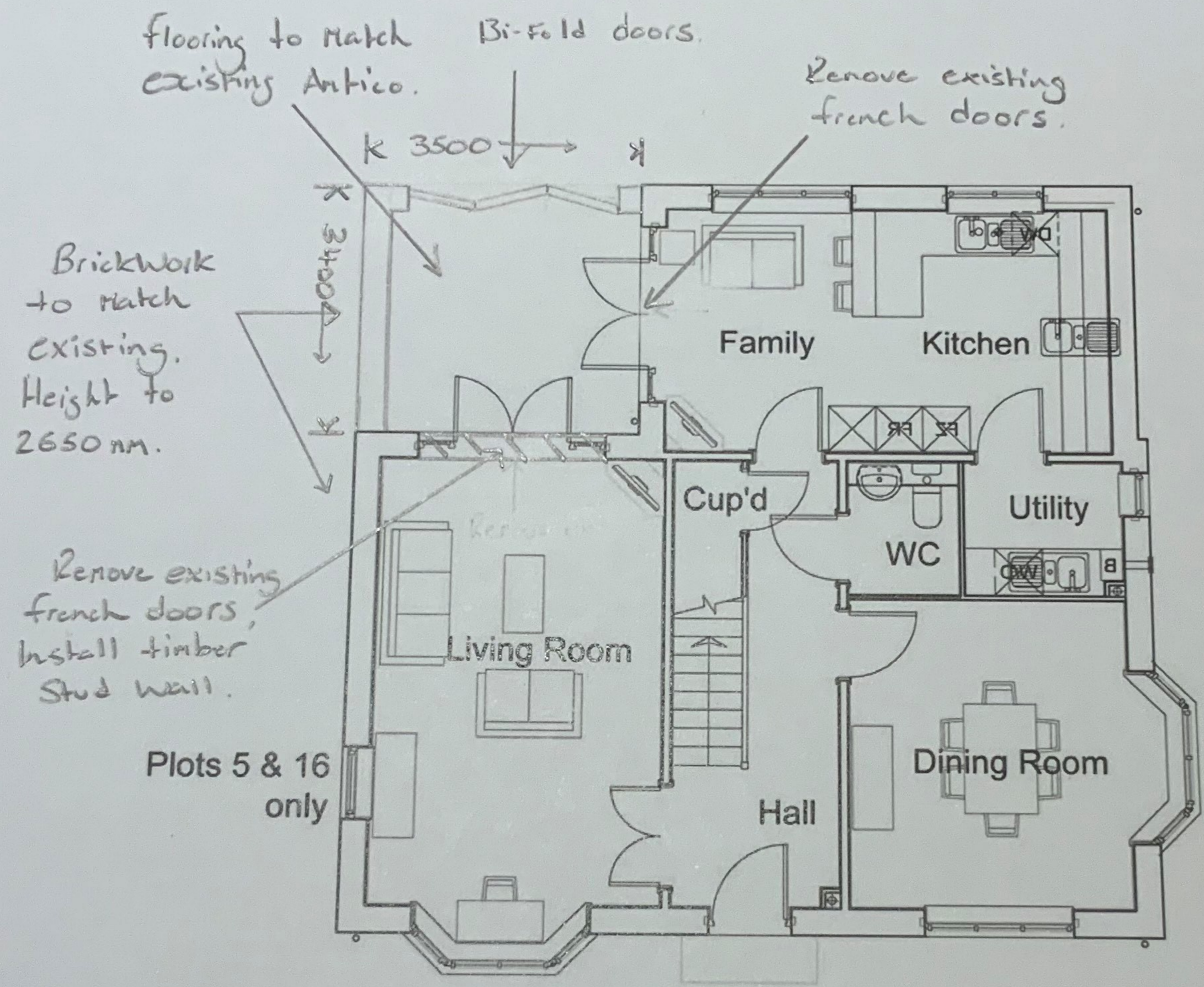
Proposed Ground Floor Plan House Type H3
