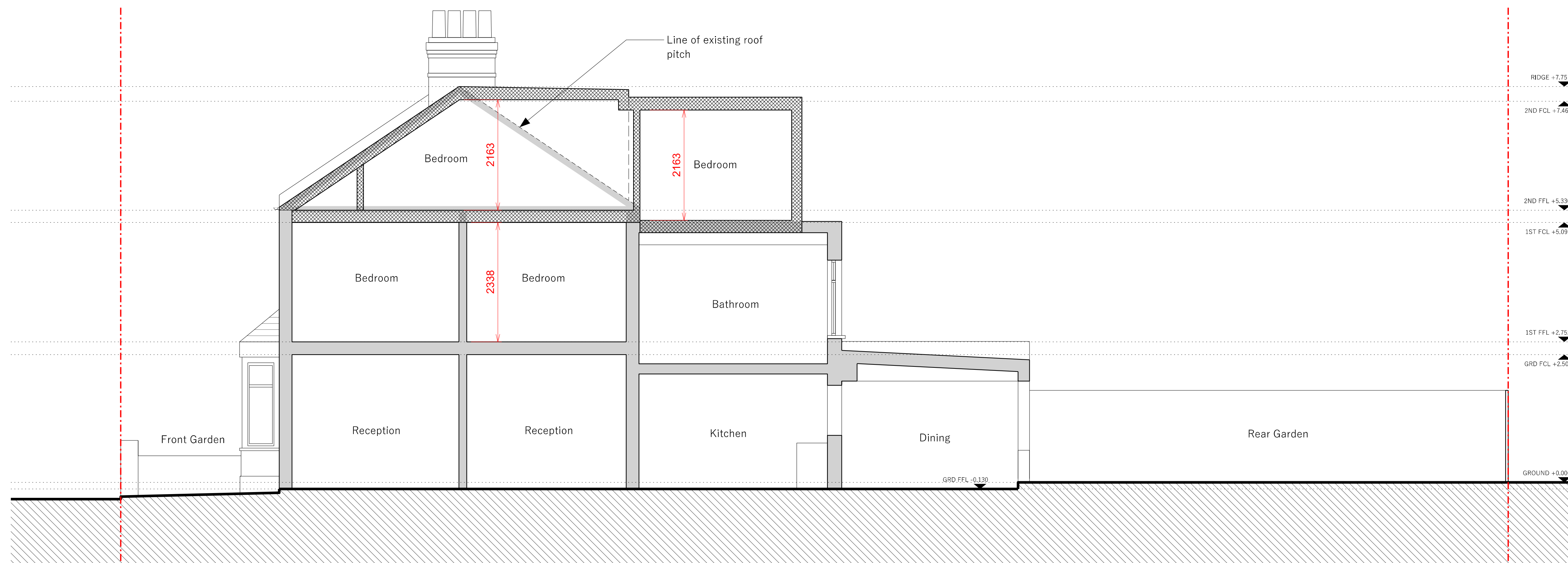
Proposed Long Section
