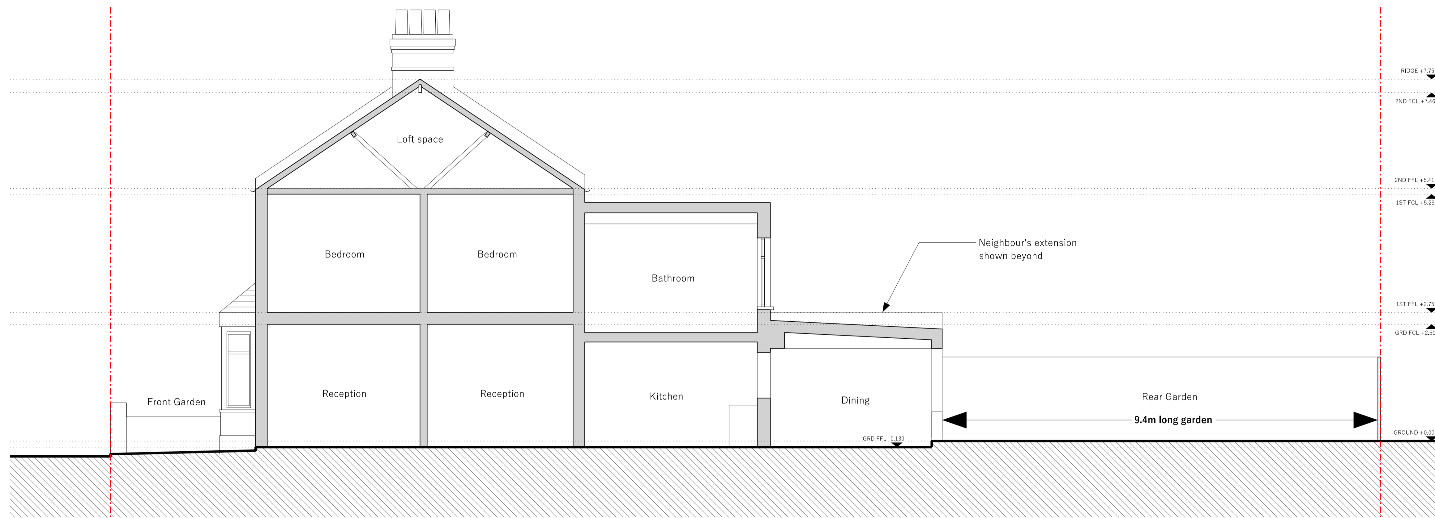
Existing Long Section
