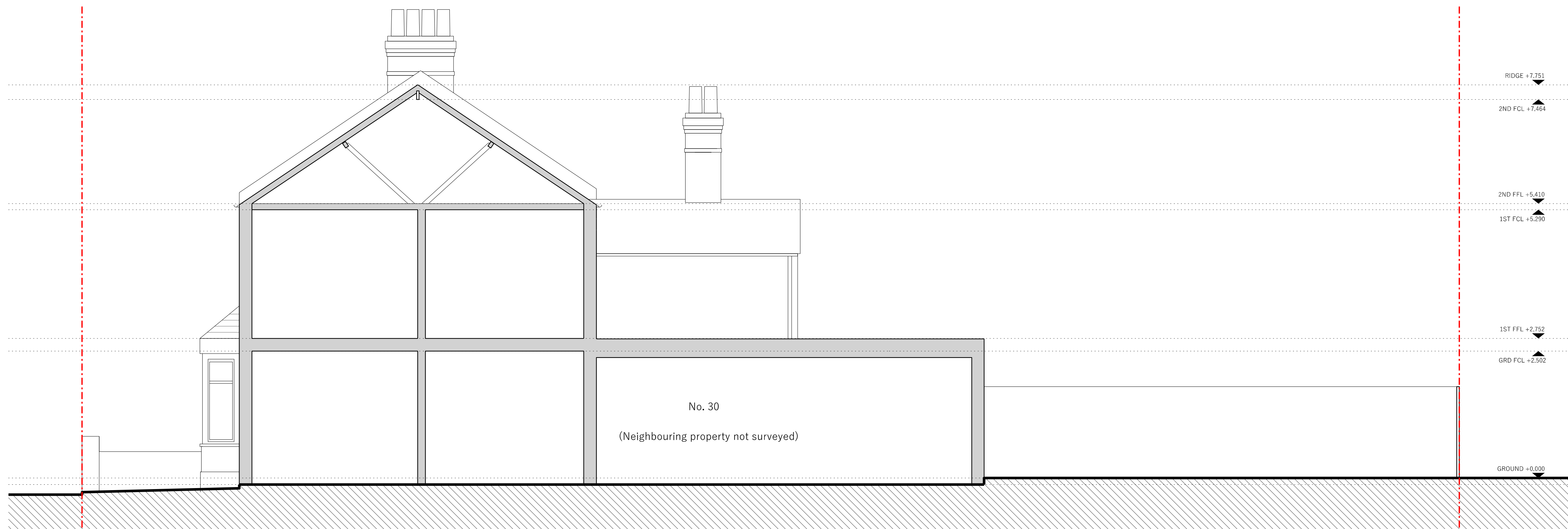
Existing Long Side Section
