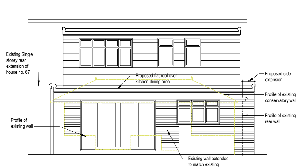
REAR/NORTH-EAST ELEVATION
