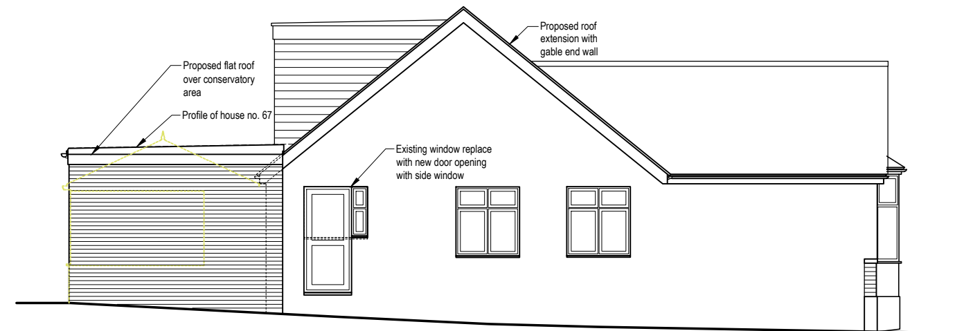
NORTH-WEST ELEVATION
