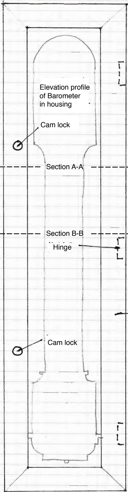
Elevation Scale 1:5 @ A4
