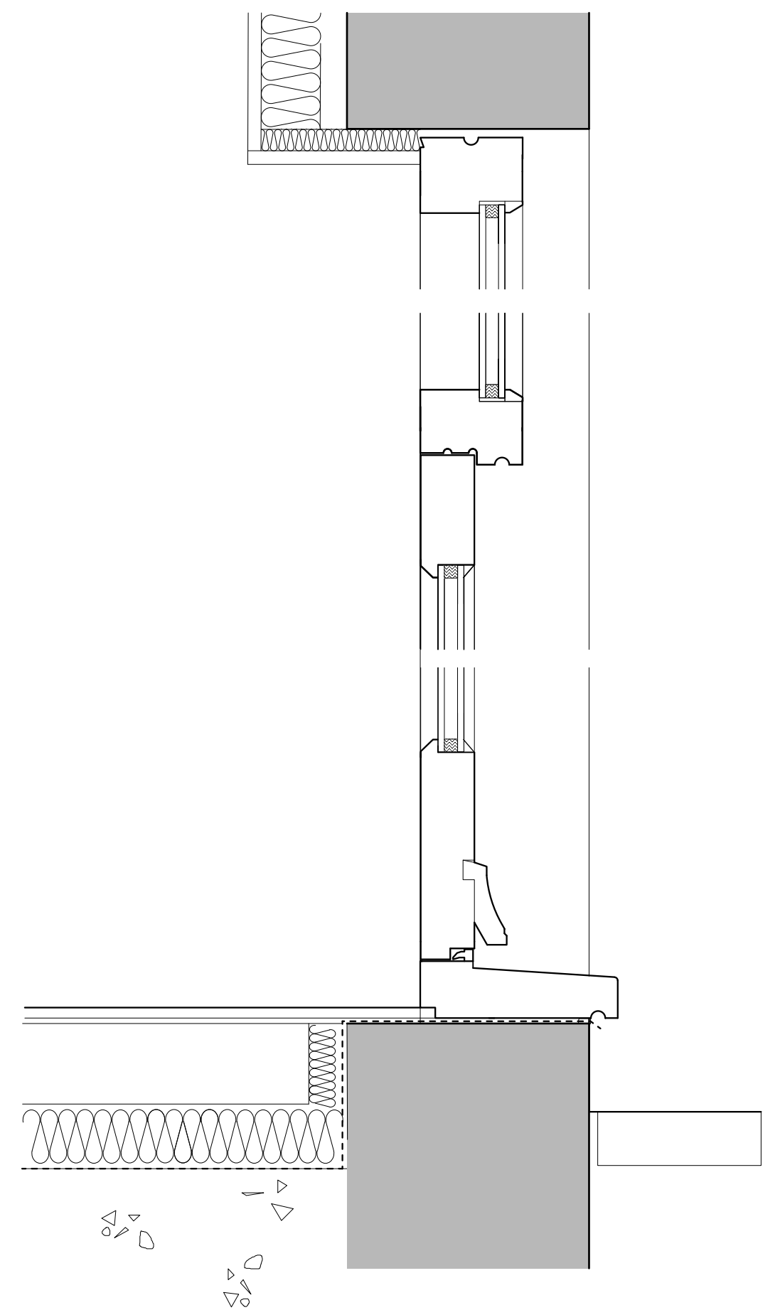
Detail B 1:5 scale
