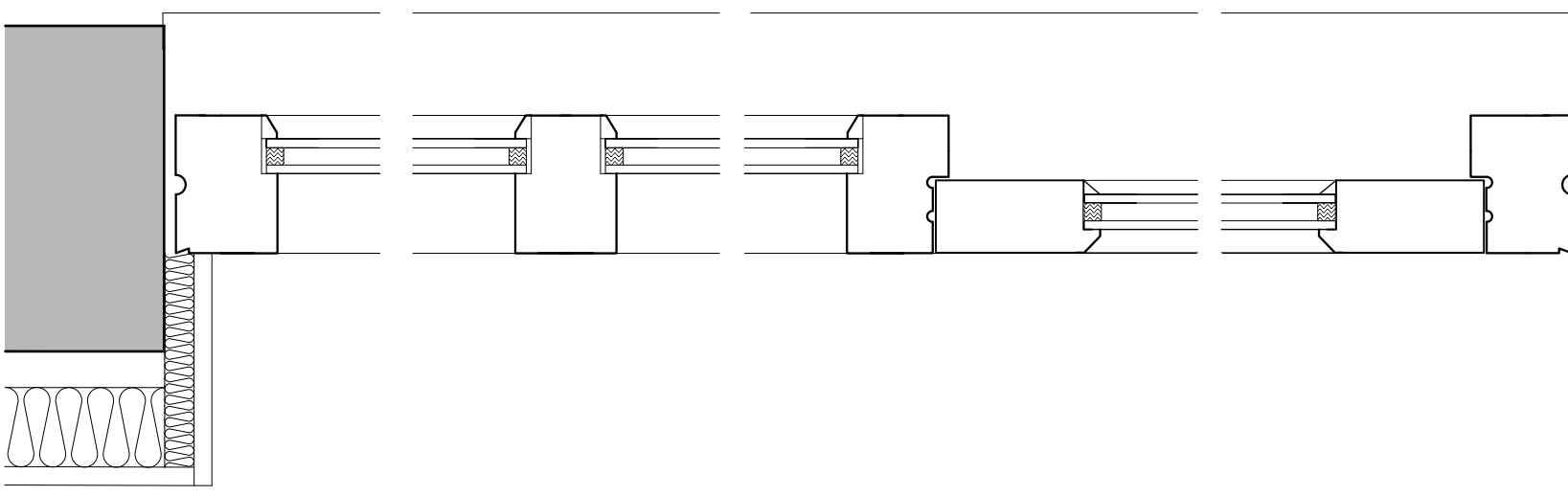
Detail A 1:5 scale
