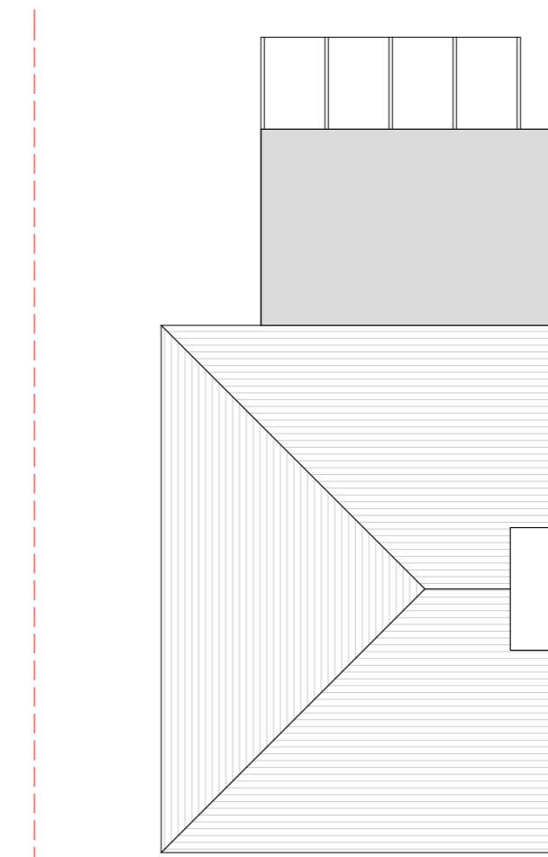
Roof Plan
