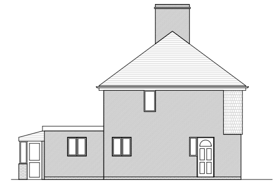
Party Wall Elevation
