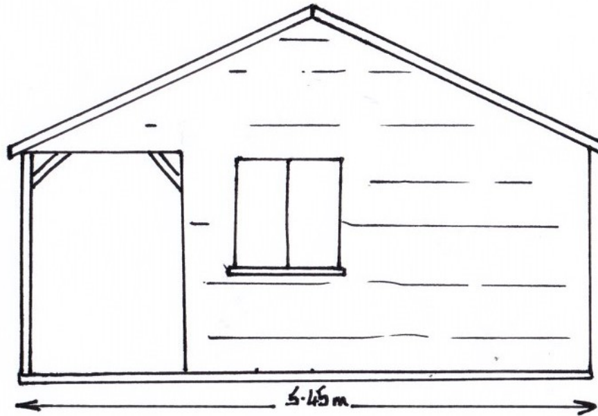
Side (West) Elevation
