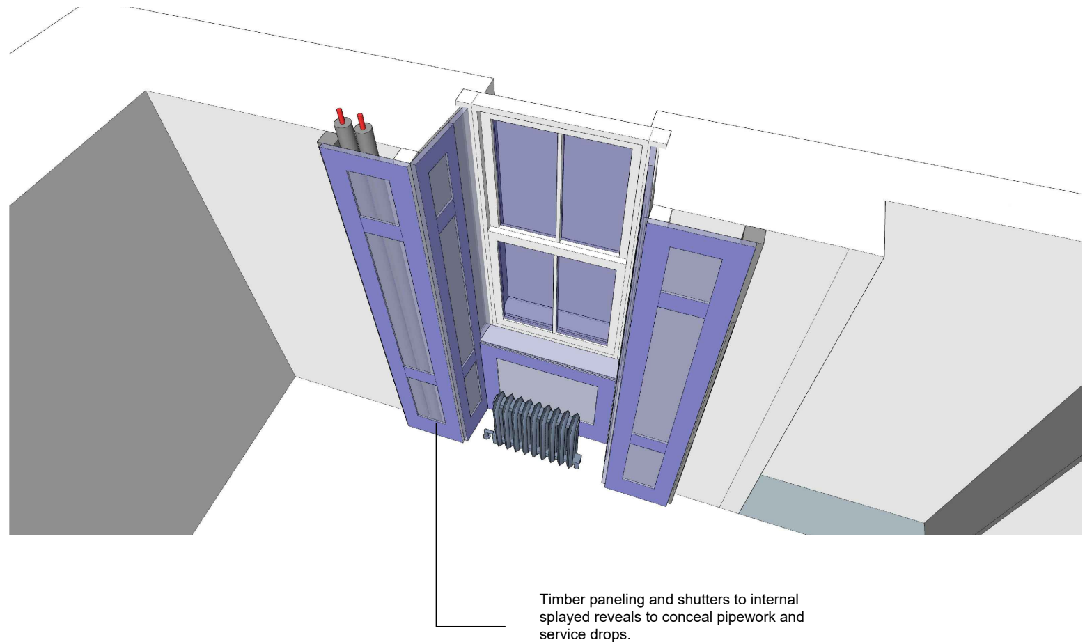
Replacement Windows A3 - 1:20 0 2500mm
