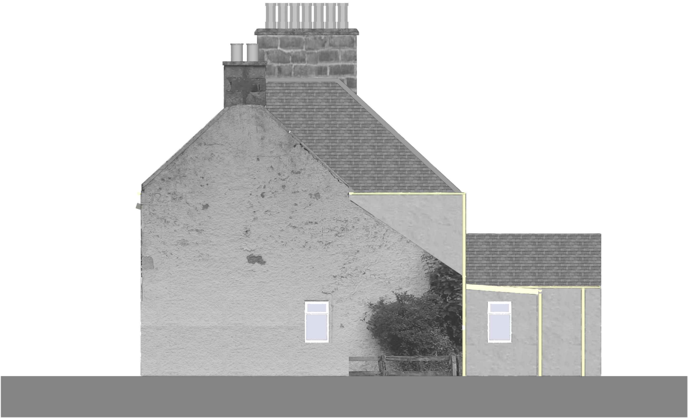
Side Elevations (West)
