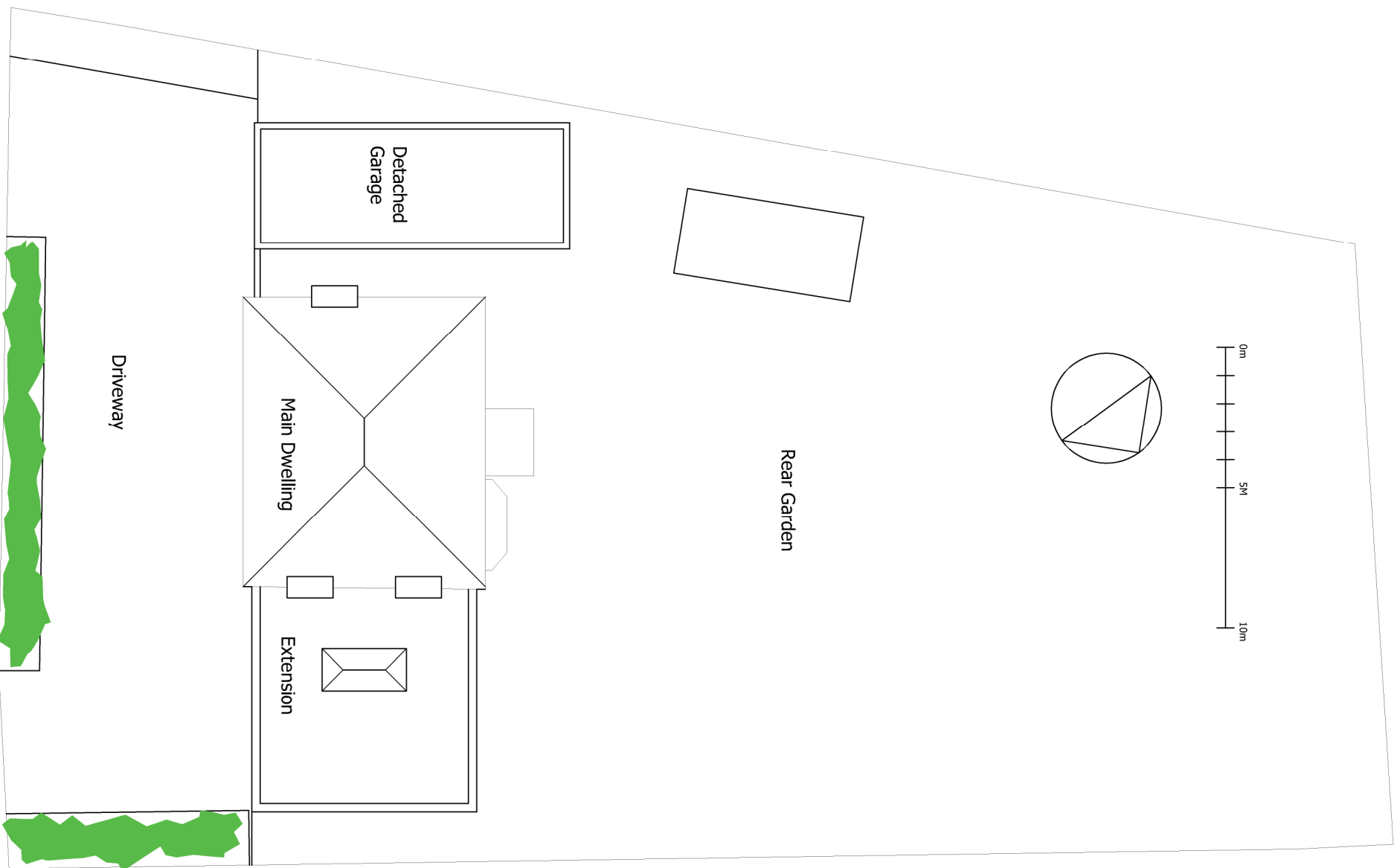
Site Plan 1:200 (A3)
