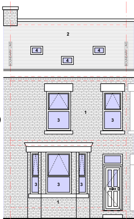
PROPOSED GA FRONT ELEVATION
