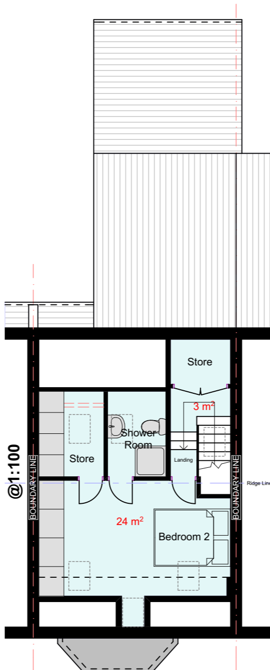
PROPOSED GA SECOND FLOOR PLAN
