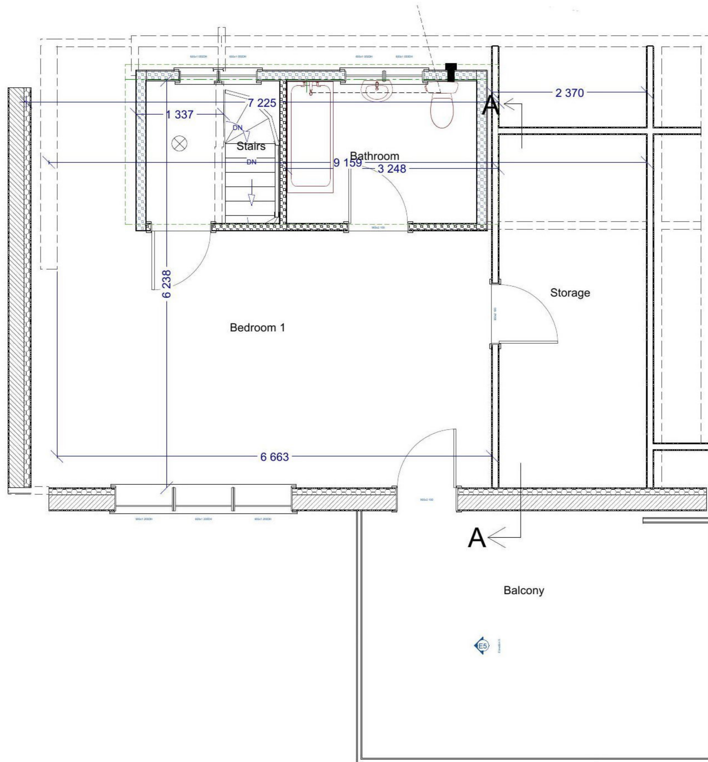
PROPOSED SECOND FLOOR PLAN SCALE 1:50
