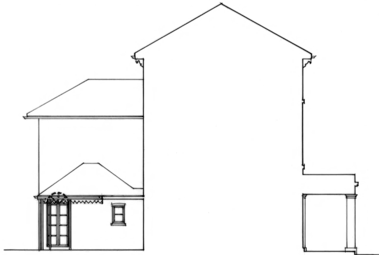
SIDE ELEVATION
