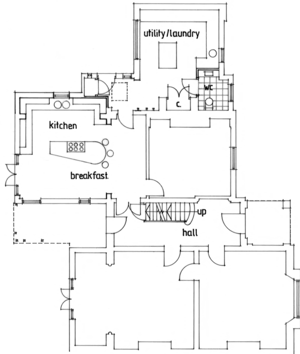
GROUND FLOOR
