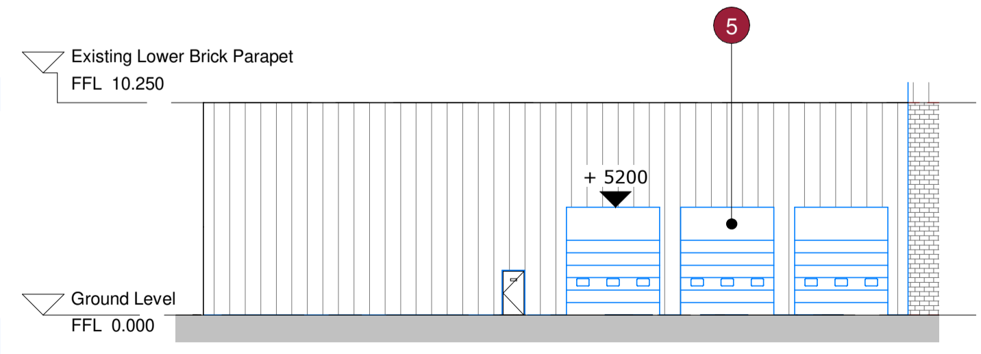
Proposed Demolition and Construction Elevation 01 1 : 250
