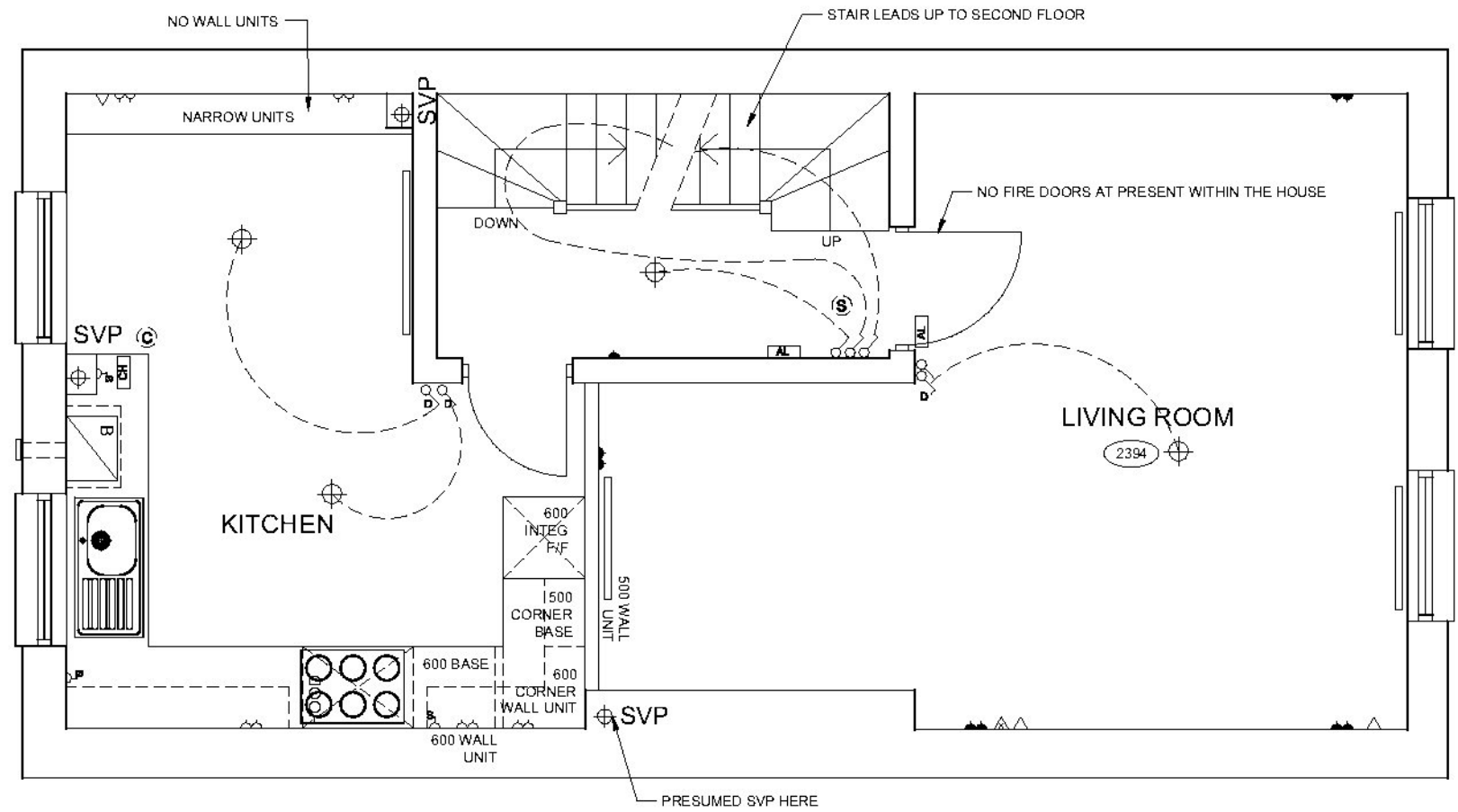
EXISTING FIRST FLOOR PLAN 1:50
