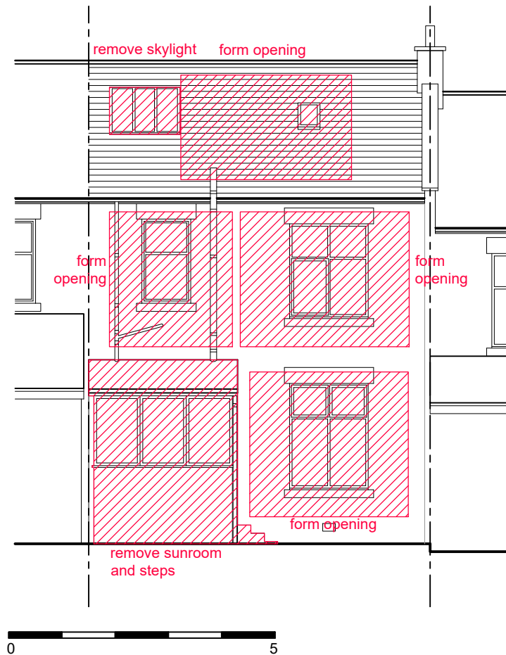
02 South elevation as existing 1:100 @ A3
