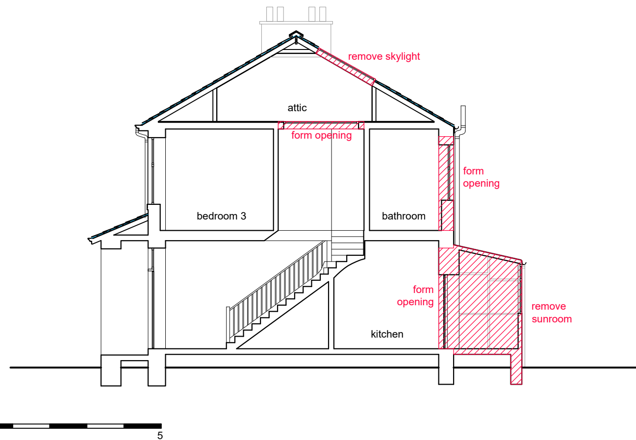
04 Section B-B' as existing 1:100 @ A3
