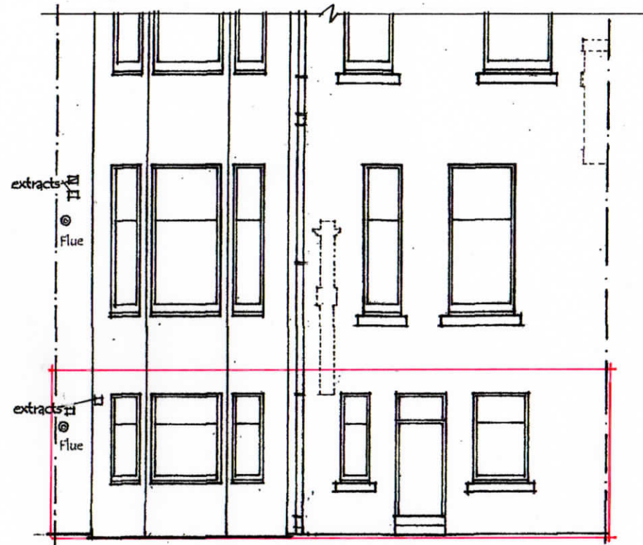
Part Rear Elevation as Existing 1:100
