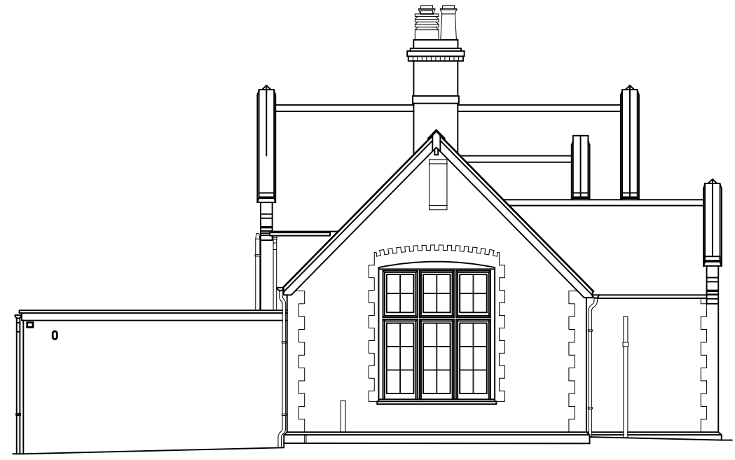
West Elevation
