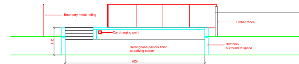
Proposed Elevation
