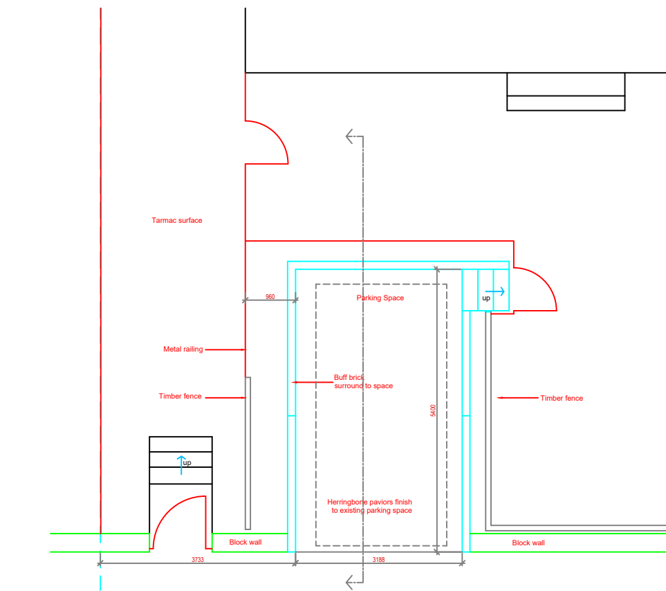
Existing Plan
