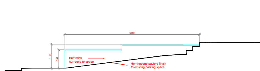
Proposed Section
