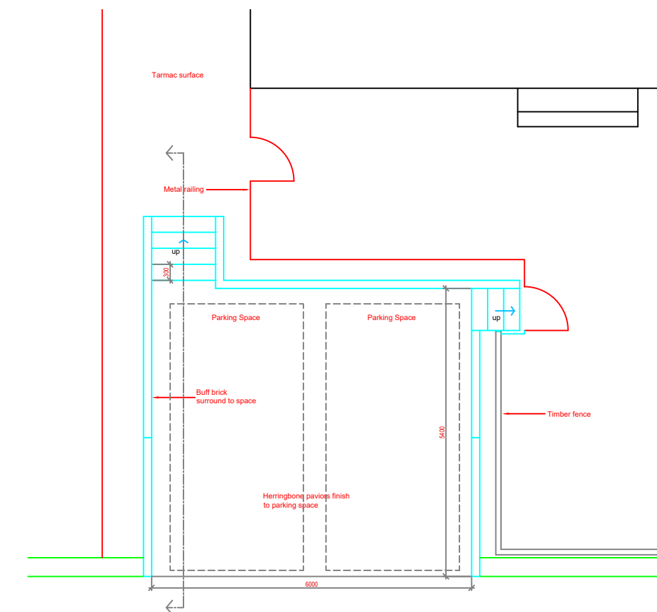
Proposed Plan
