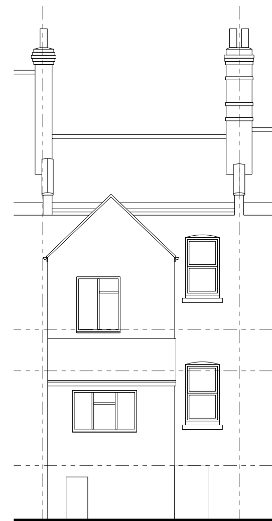
REAR ELEVATION
