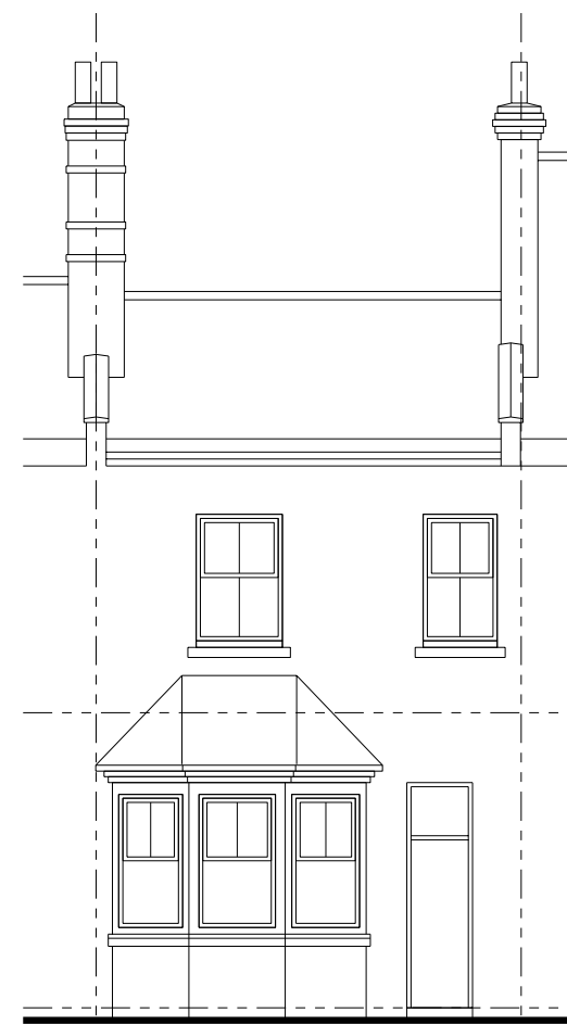
FRONT ELEVATION
