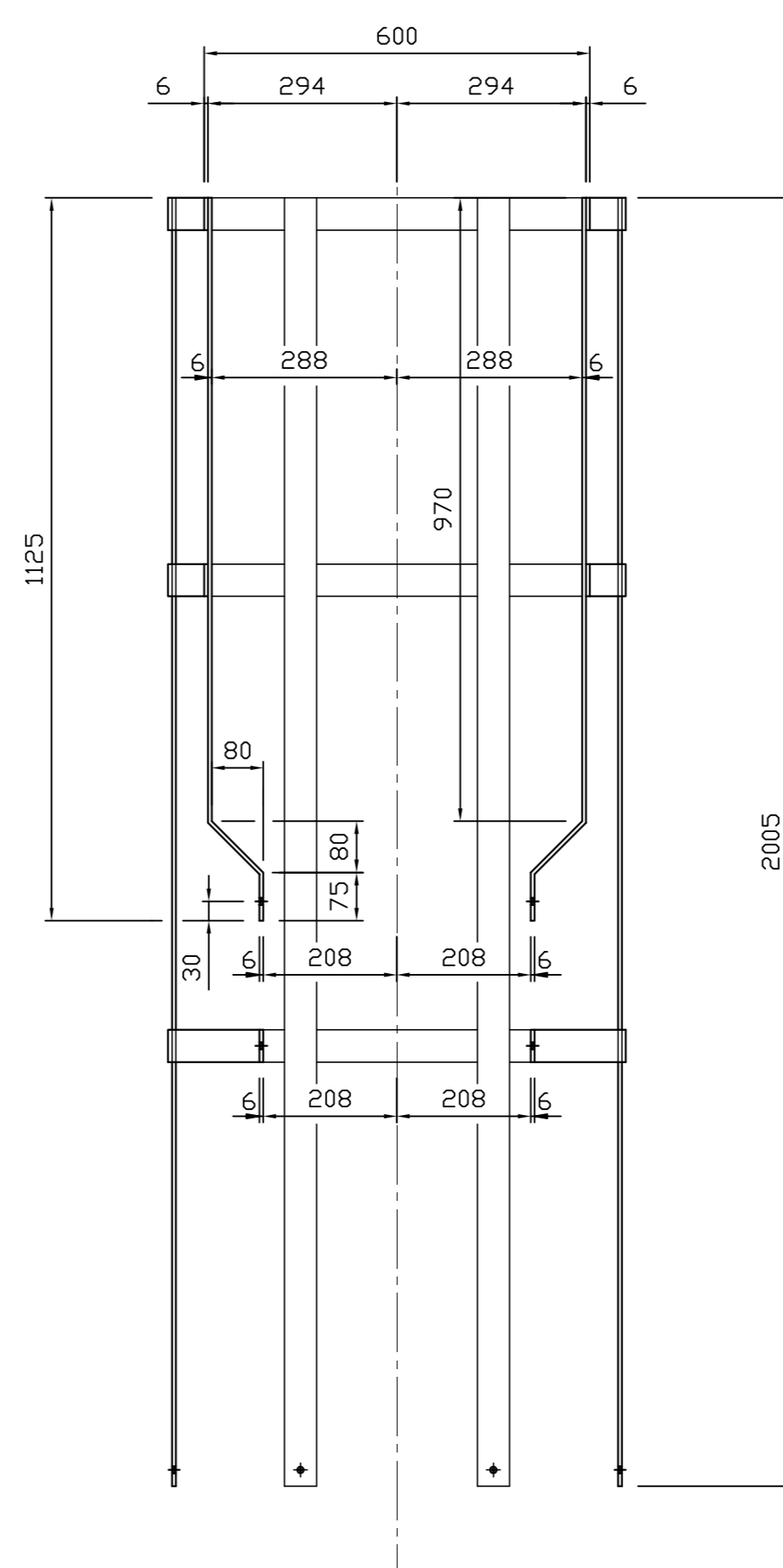
Section on G-G
