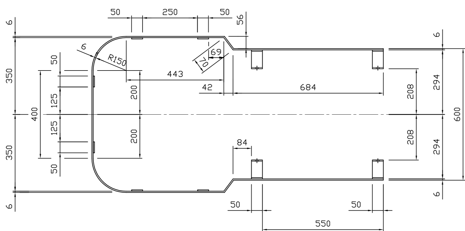
Plan on D-D
