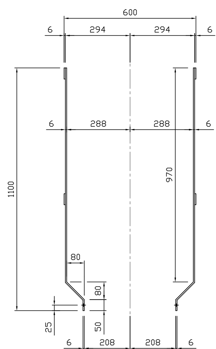
View on F-F
