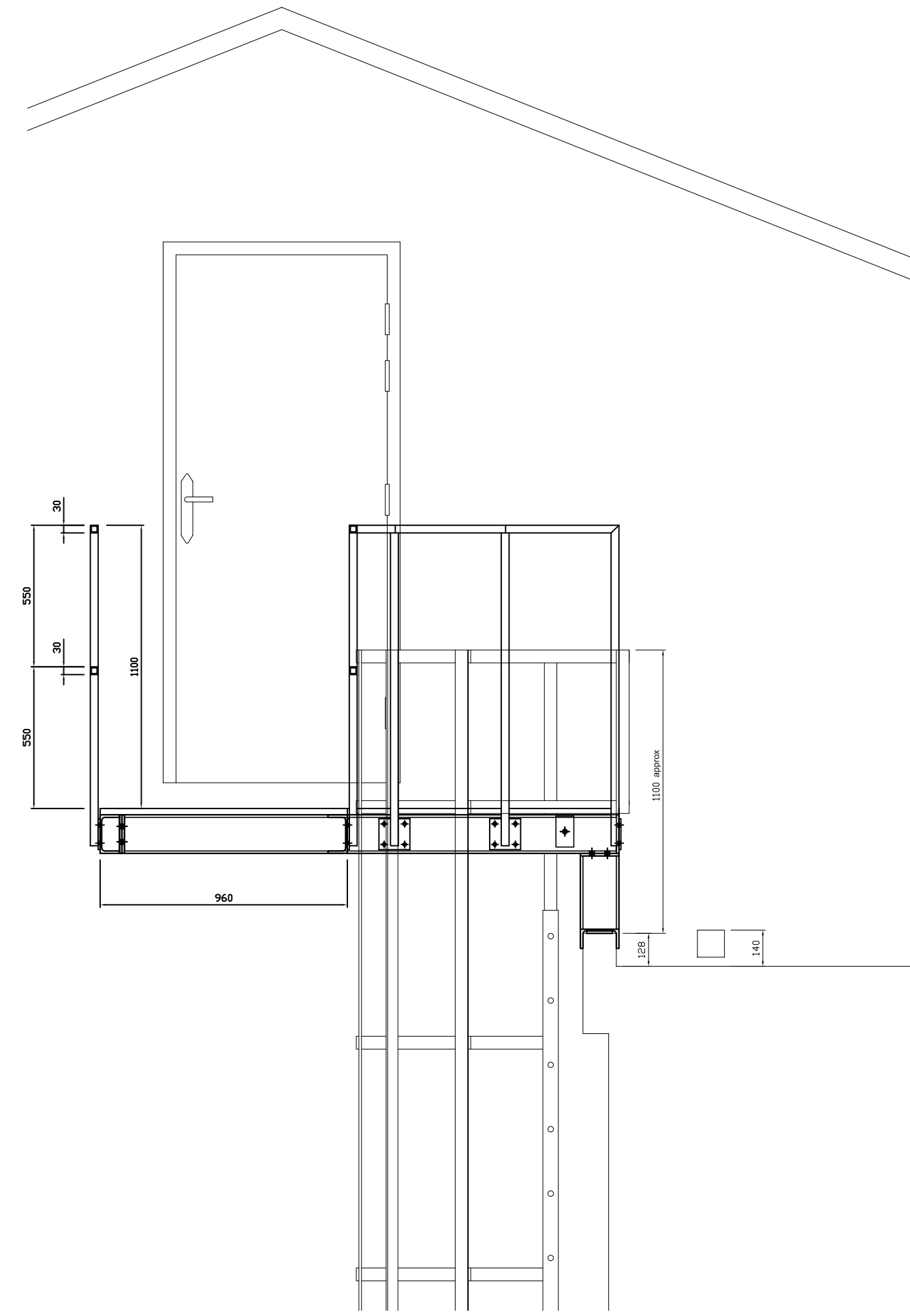
Section B-B
