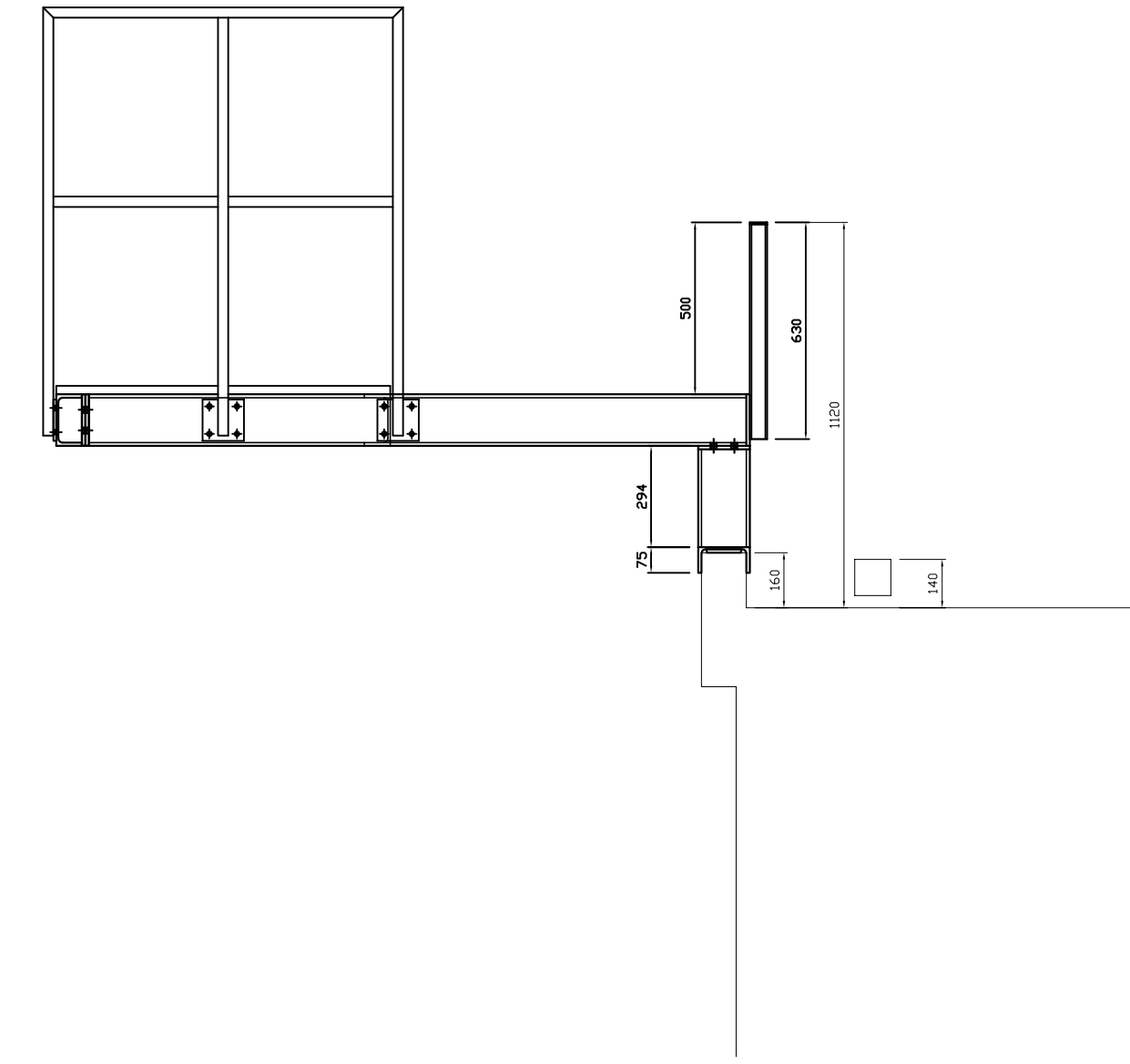
Section C-C
