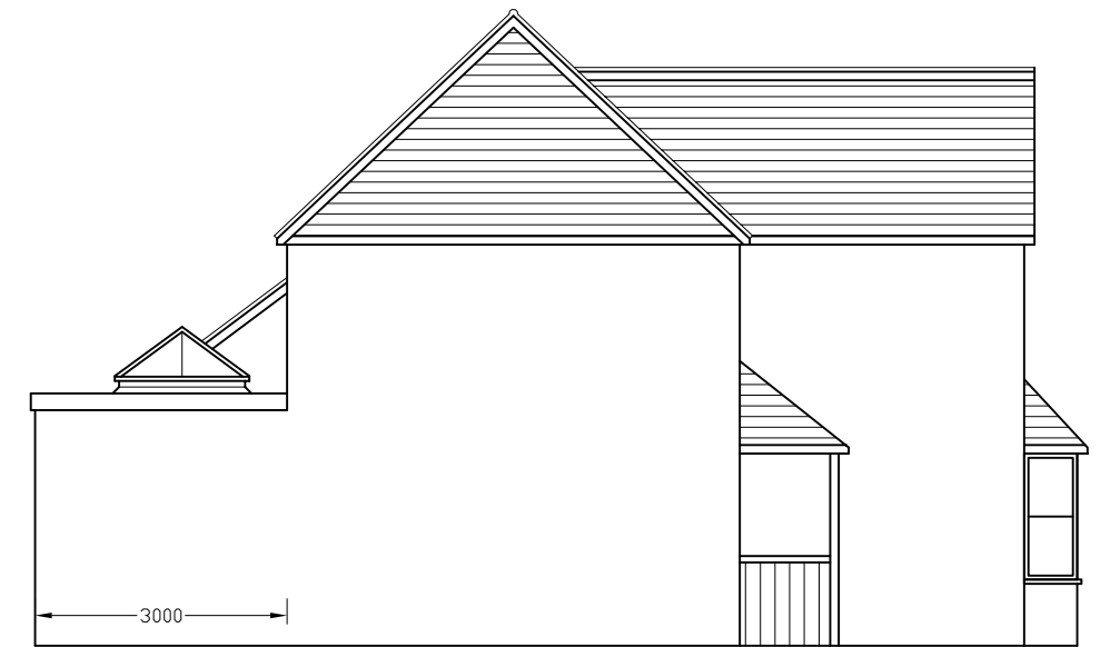
PROPOSED SIDE ELEVATION materials to match existing
