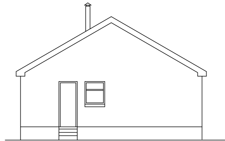
NORTH ELEVATION
