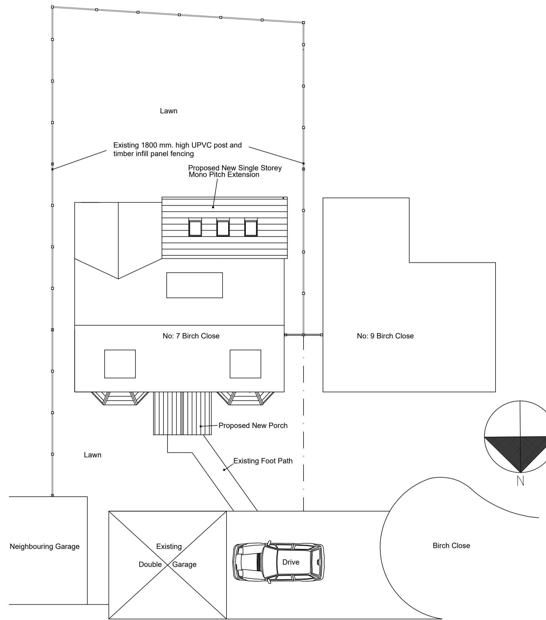
Proposed Site Plan 1:100
