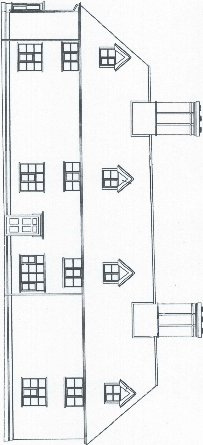
EAST (FRONT) ELEVATION
