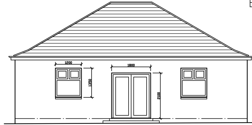
REAR (SOUTH EAST) ELEVATION
