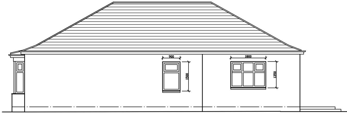
FRONT (NORTH WEST) ELEVATION
