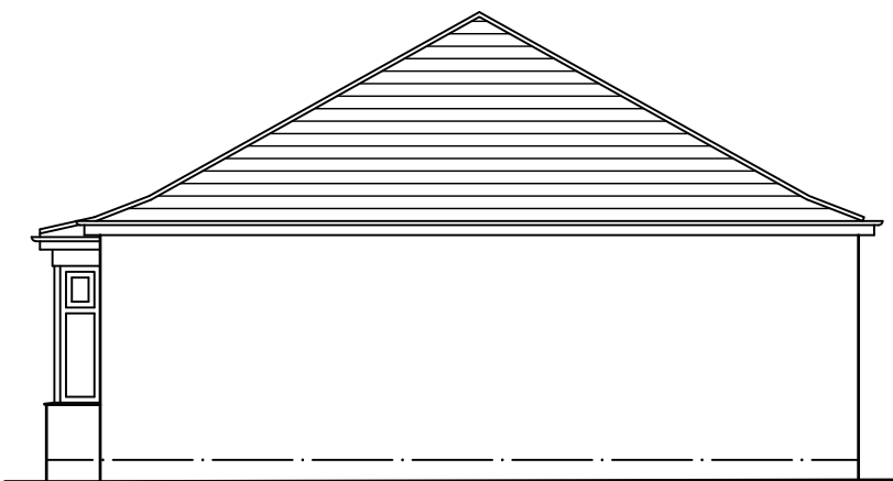
SIDE (SOUTH WEST) ELEVATION
