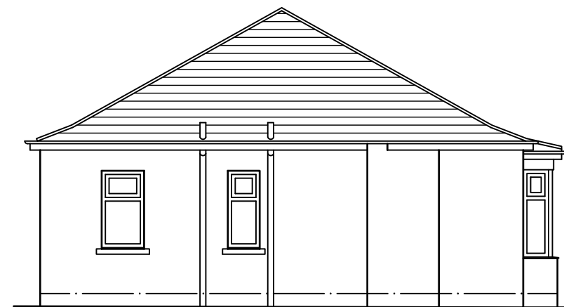
SIDE (NORTH EAST) ELEVATION
