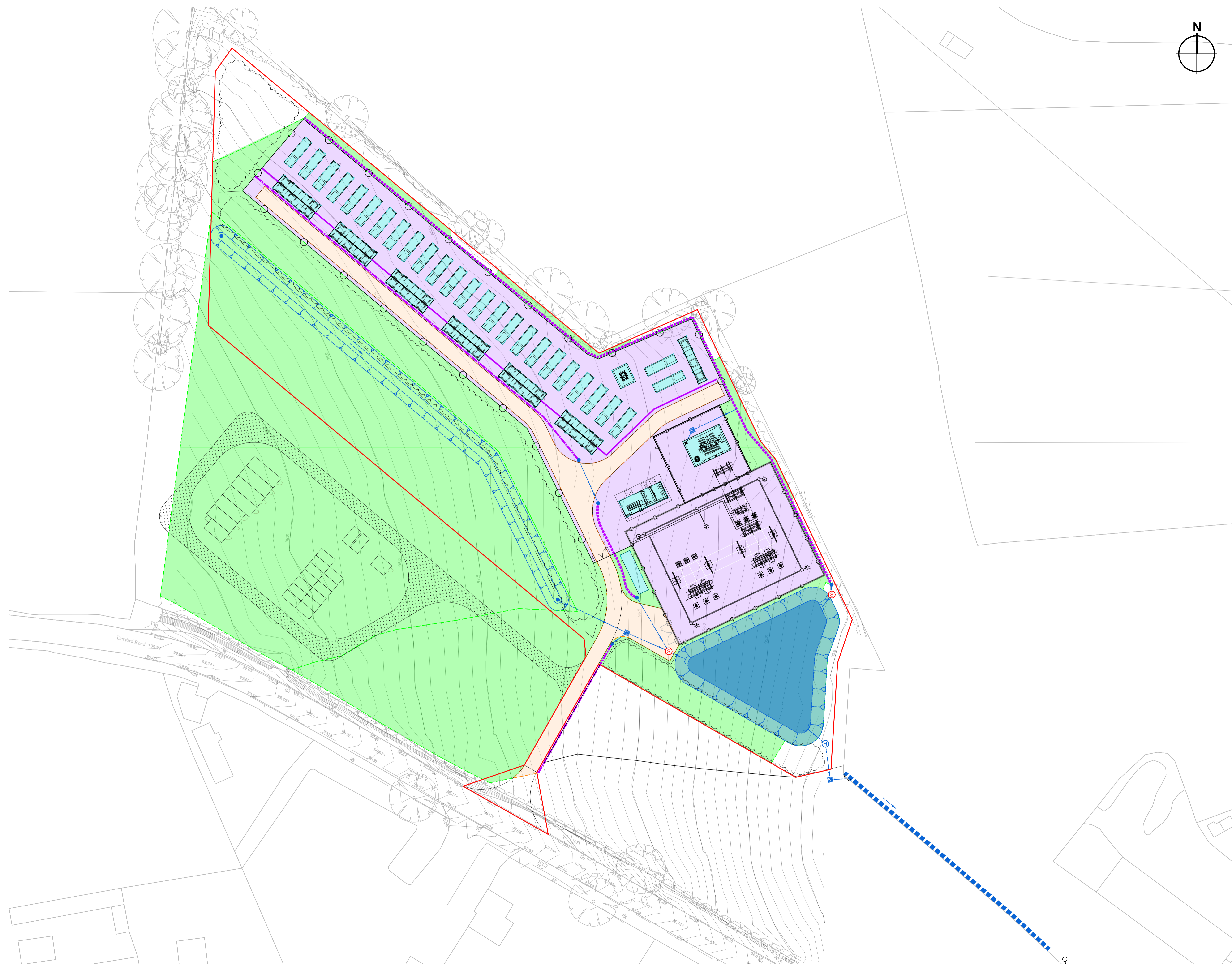
10m SCALE 1:500
