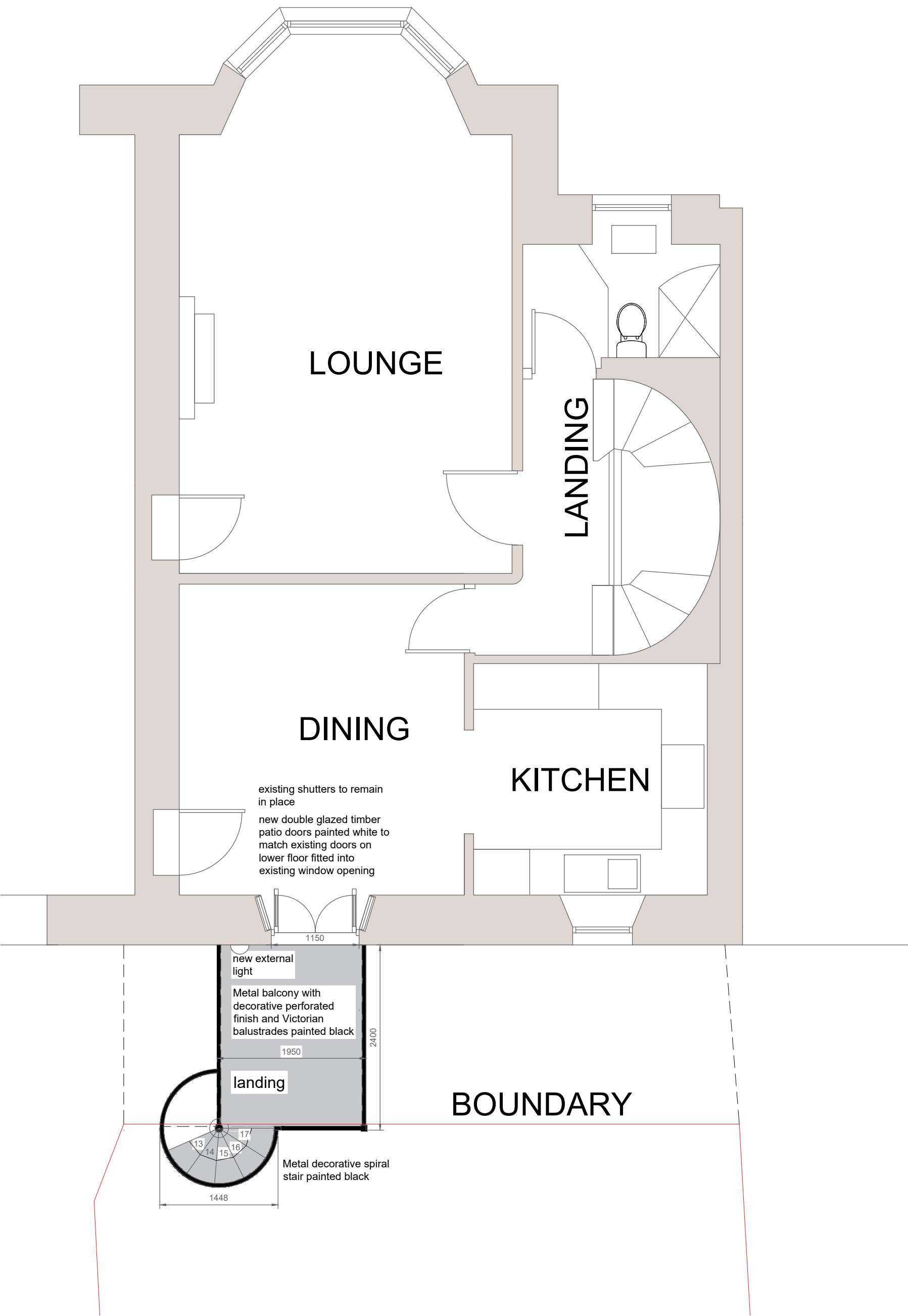
PROPOSED SPIRAL STAIR
