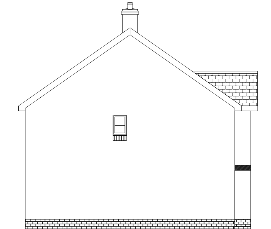
South Elevation
