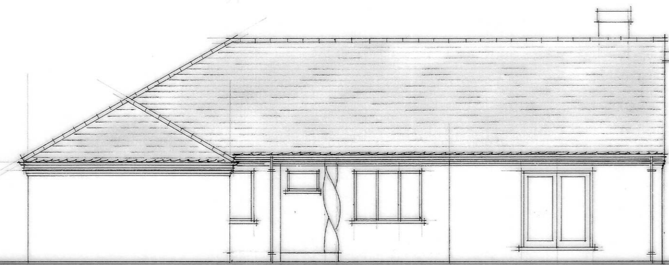
SIDE - WEST
