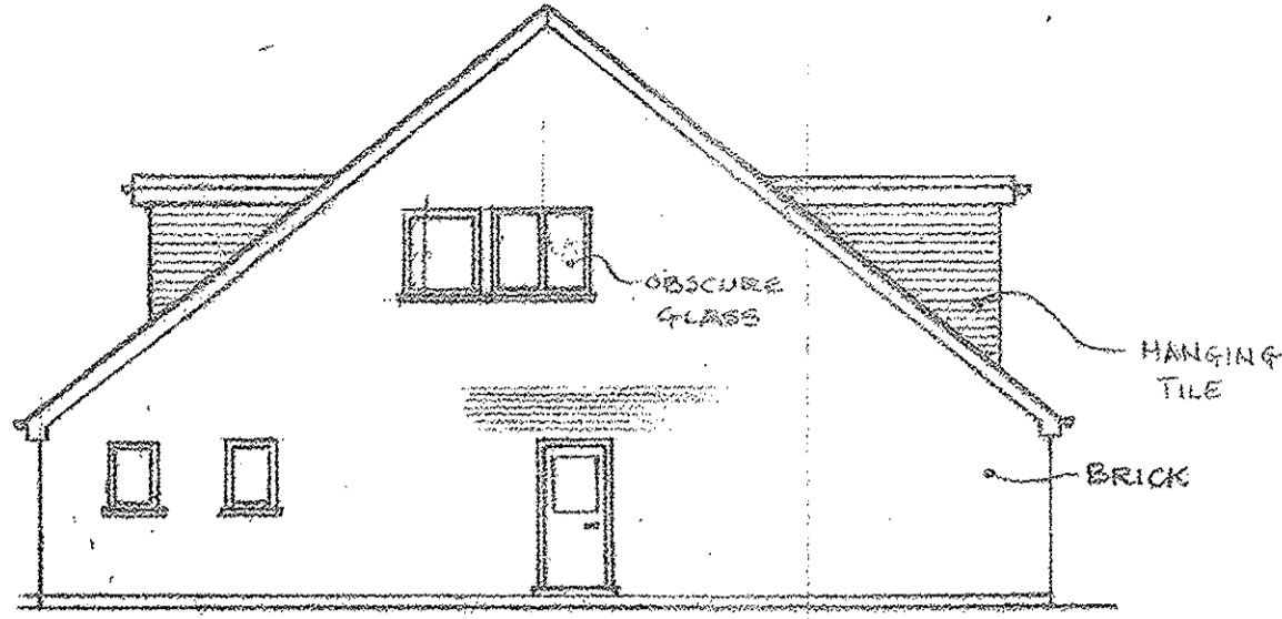
SIDE VIEW (EAST)
