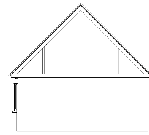
SECTION Scale 1:100
