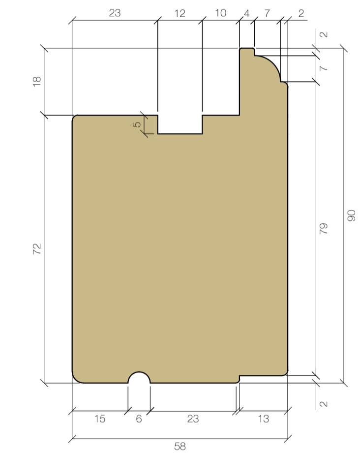
STILE 58x90 FINISH SIZE
