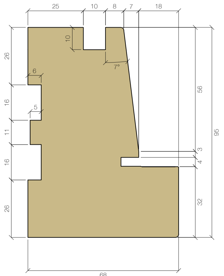
CILL 95x68 FINISH SIZE
