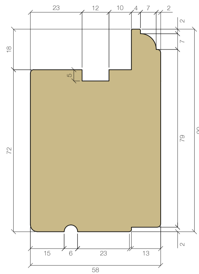
TOP RAIL 58x90 FINISH SIZE
