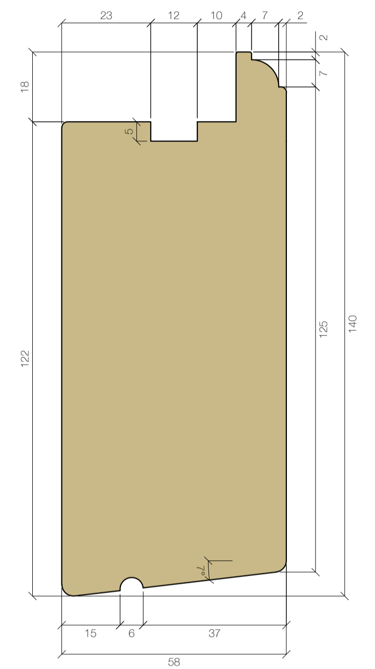
BASE RAIL 58x140 FINISH SIZE
