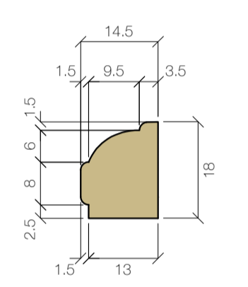
BEADING 14.5x18 FINISH SIZE
