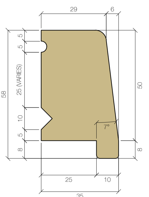
NOSING 58x35 (TYPICAL) FINISH SIZE
