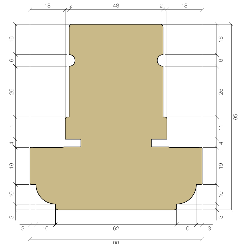
MULLION 95x88 FINISH SIZE
