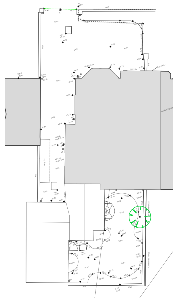
EXISTING SITE PLAN WITH PART ROOF PLAN
